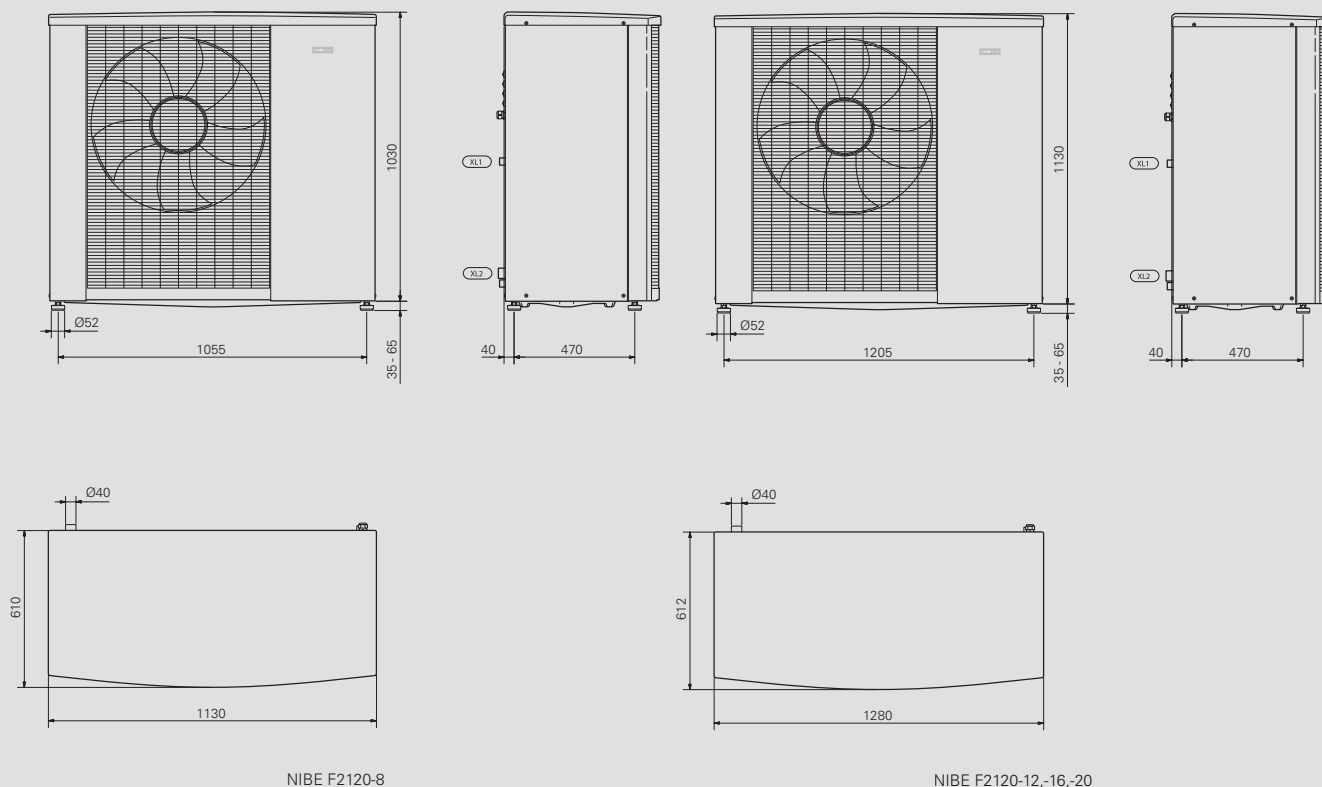
NIBE F2120-8
